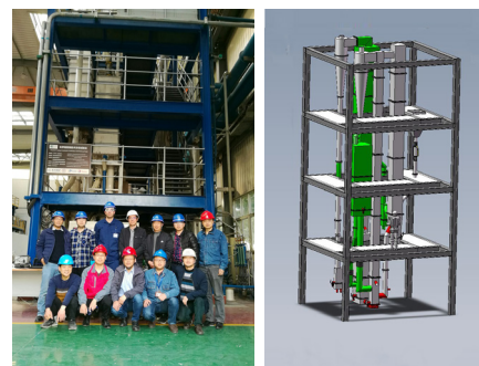
1.5 MWth model of the whole loop operated for different solid and gas flow conditions.
