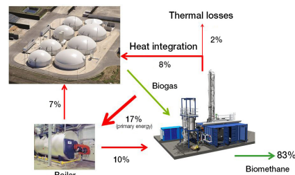
Thermal integration and use of the new IFPEN solvent (source: Arol Energy).
