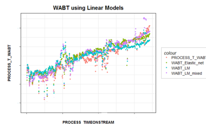
Average reactor temperature (WABT c ) as a function of time on stream (TOS) (Process_T_WABT = measured temperature).
